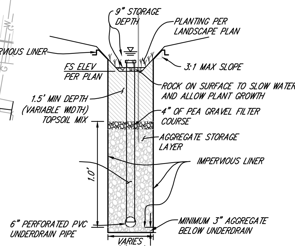
BIOFILTRATION BASIN B SECTION TYPICAL SECTION NOT TO SCALE
