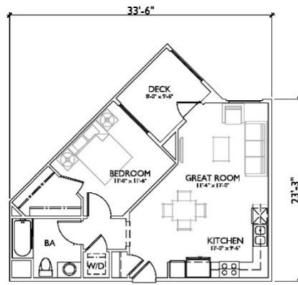
PLAN 1: 1BD/1BA TOTAL 620 S.F. DECK 75 S.F.
