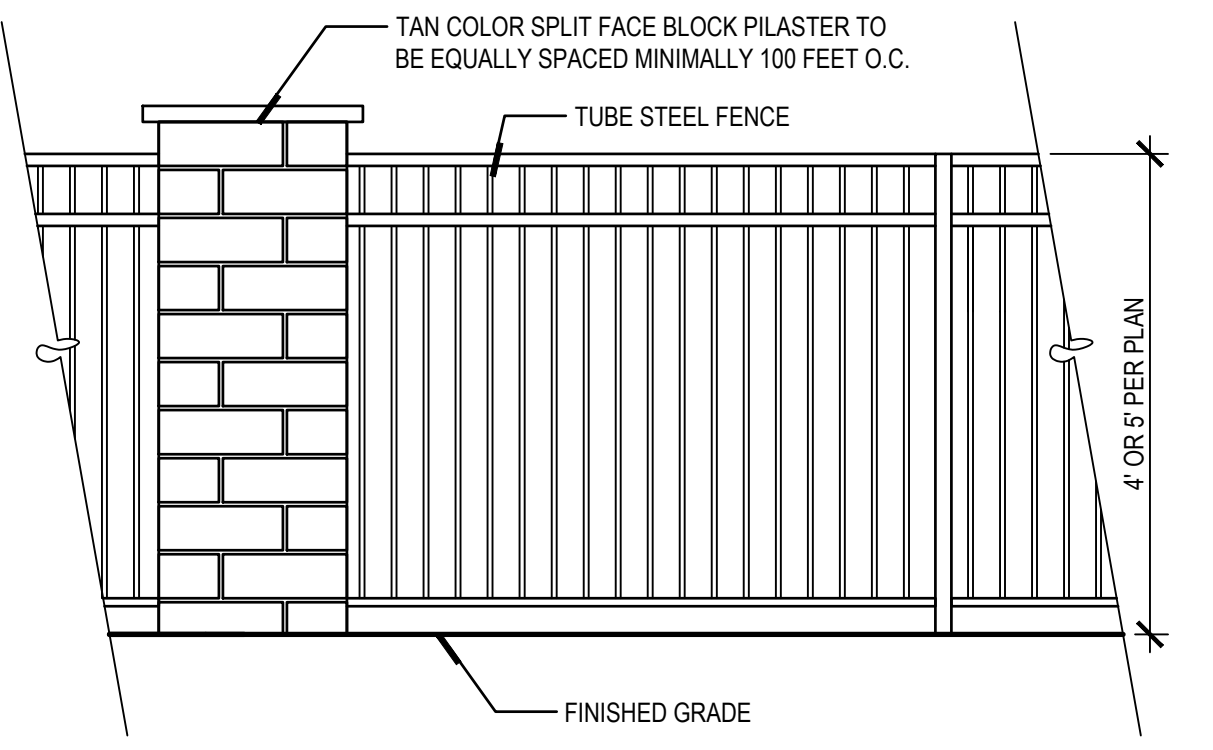
A TUBULAR STEEL FENCE
