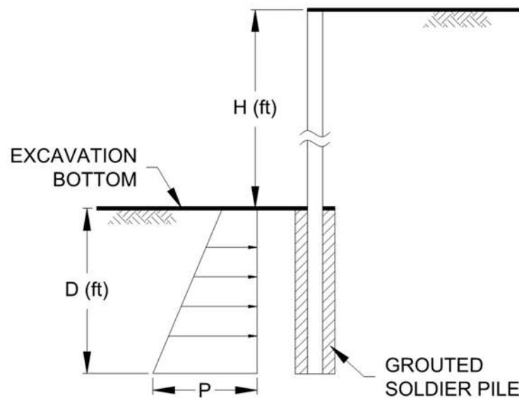
Passive Pressures on Shoring
