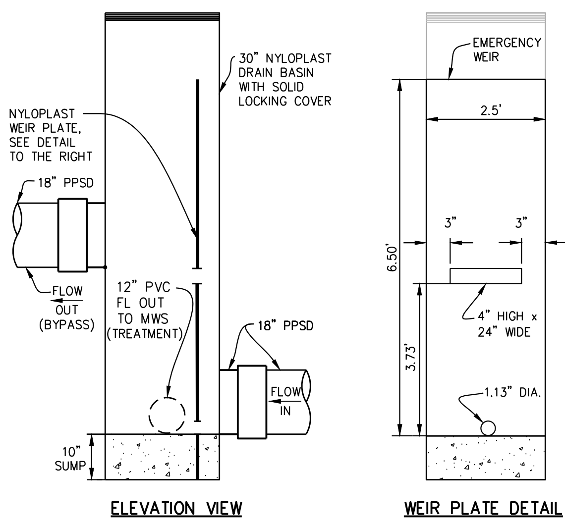
DETENTION SYSTEM UD-1 FLOW CONTROL STRUCTURE NO SCALE
