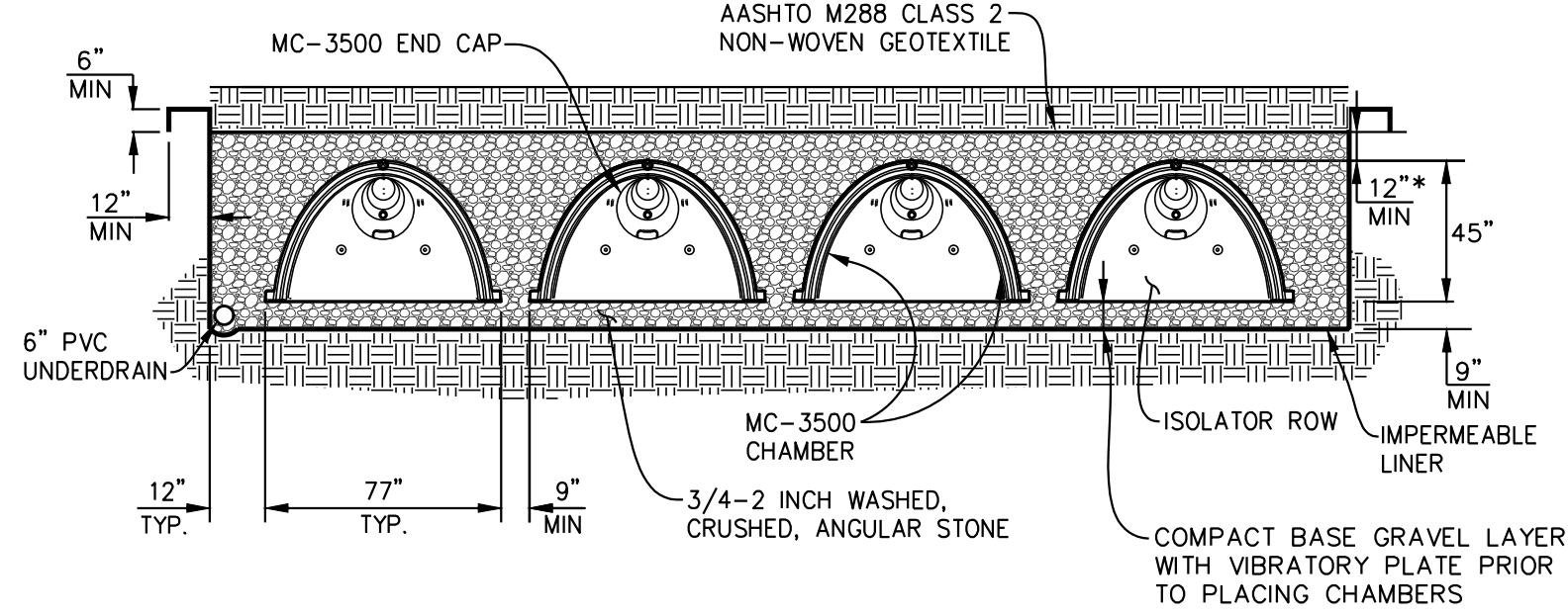
DETENTION SYSTEM "UD-2" TYPICAL CROSS SECTION
