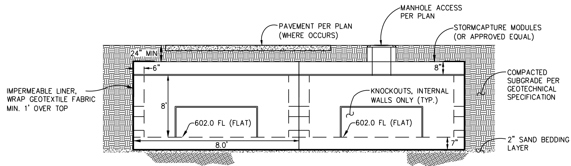
DETENTION SYSTEM "UD-1" TYPICAL CROSS SECTION
