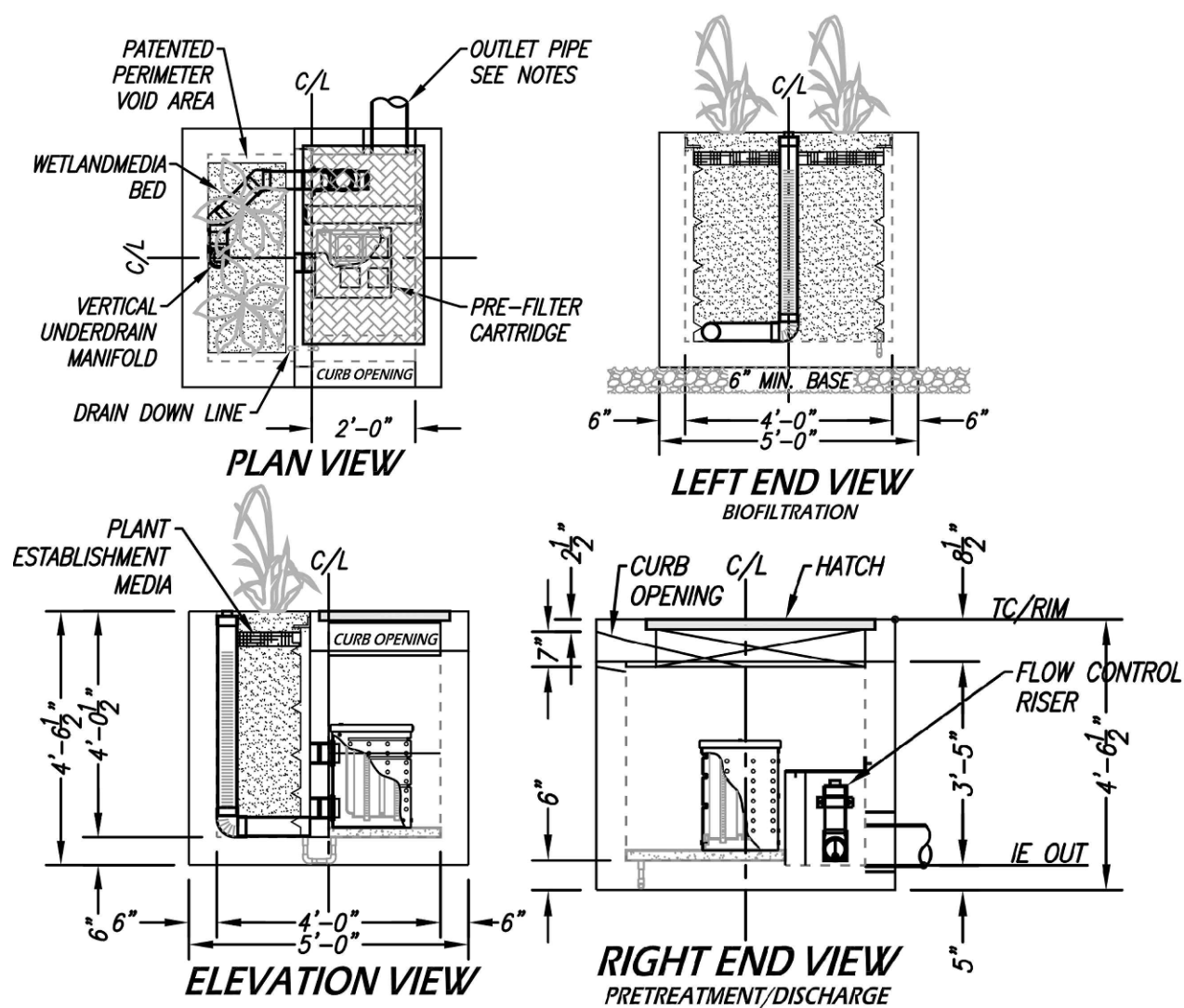
PROPRIETARY BIOFILTRATION, MODULAR WETLAND SYSTEM, OR APPROVED EQUIVALENT
