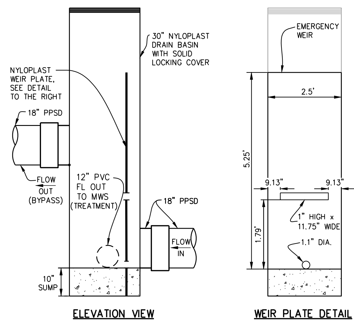
DETENTION SYSTEM UD-2 FLOW CONTROL STRUCTURE NO SCALE
