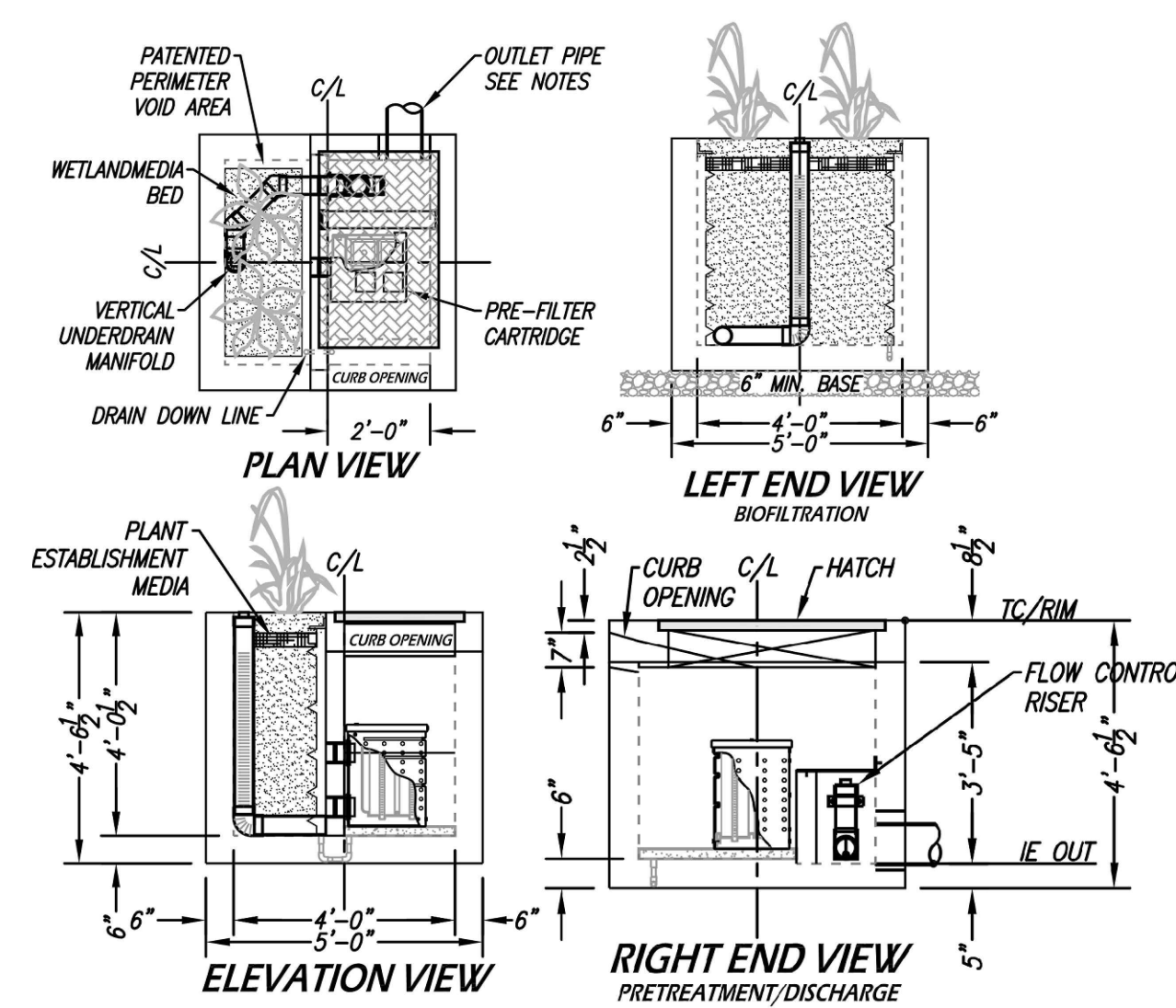
PROPRIETARY BIOFILTRATION, MODULAR WETLAND SYSTEM, OR APPROVED EQUIVALENT NO SCALE
