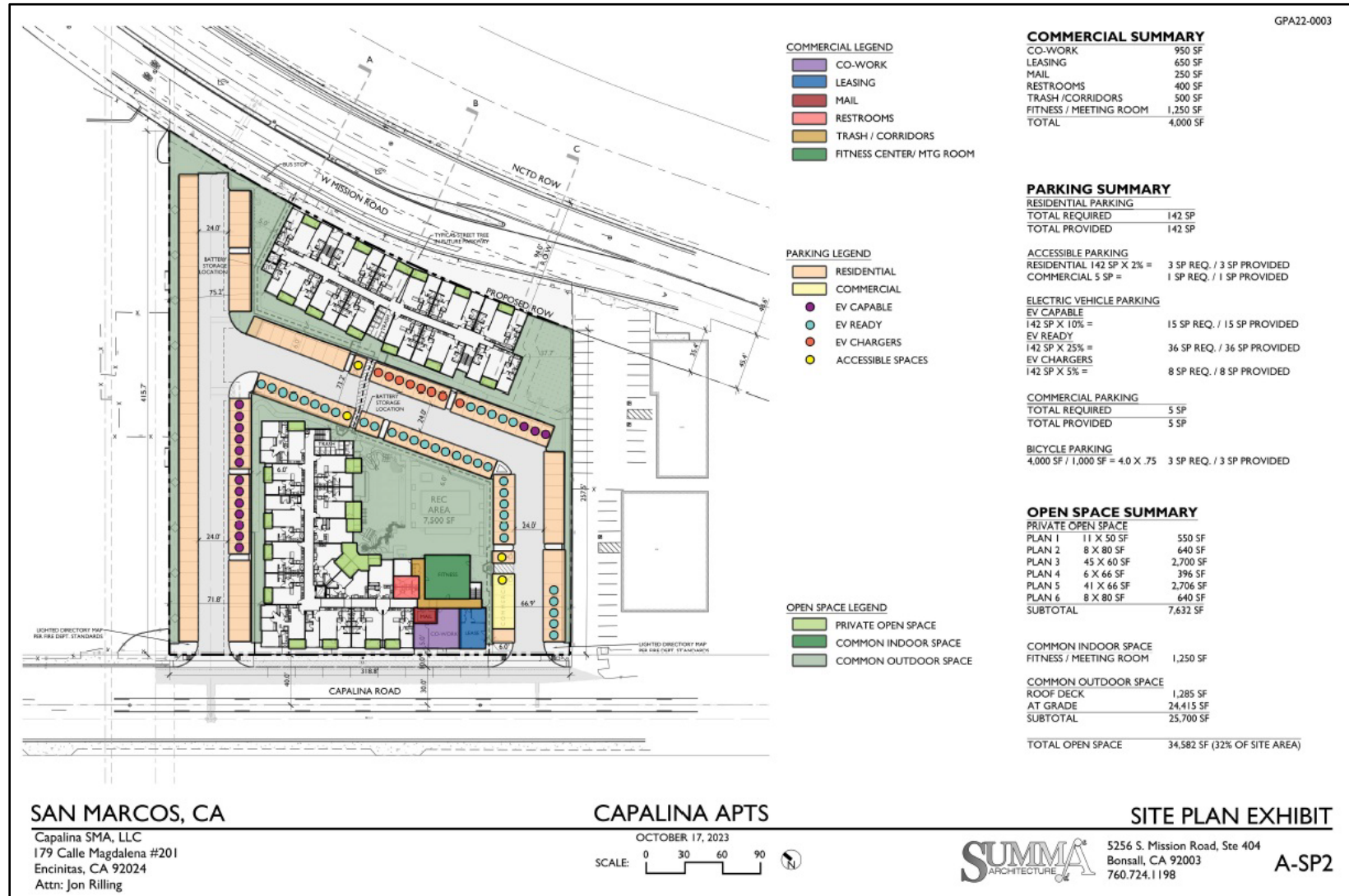
Figure 2-3. Site Plan Exhibit
