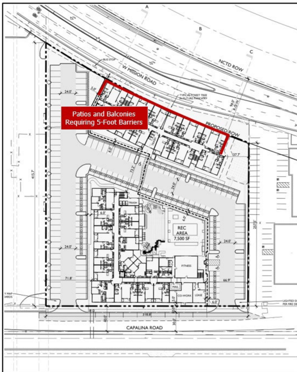
Figure 3.11-3. Area of Enhanced Shielding on Patios and Balconies
