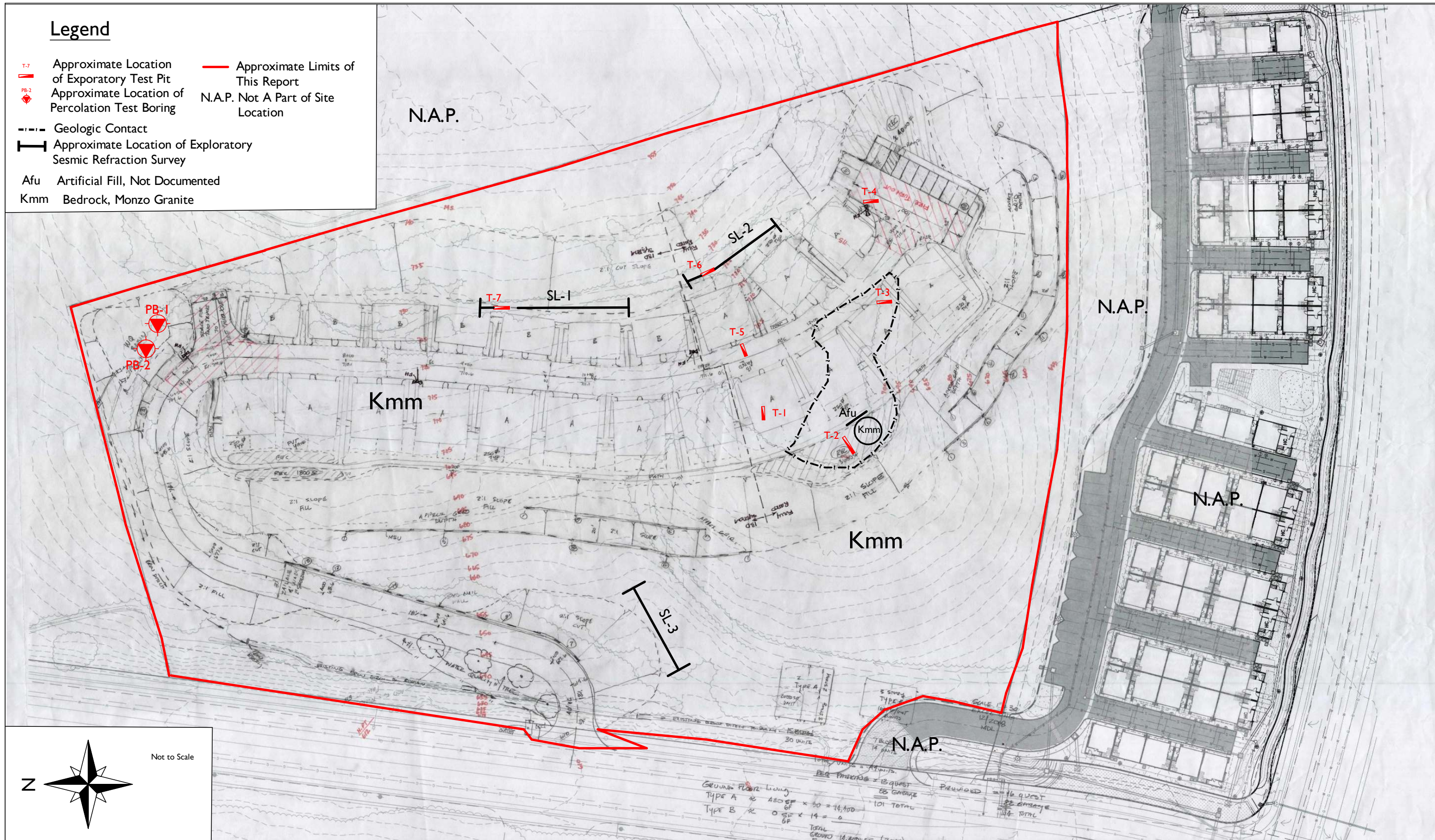
Figure 2 Geotechnical Map
