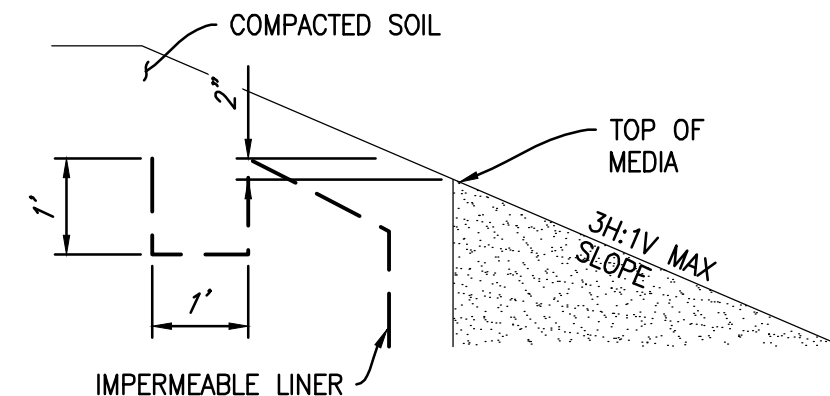
IMPERMEABLE LINER EDGE ANCHOR DETAIL NOT TO SCALE
