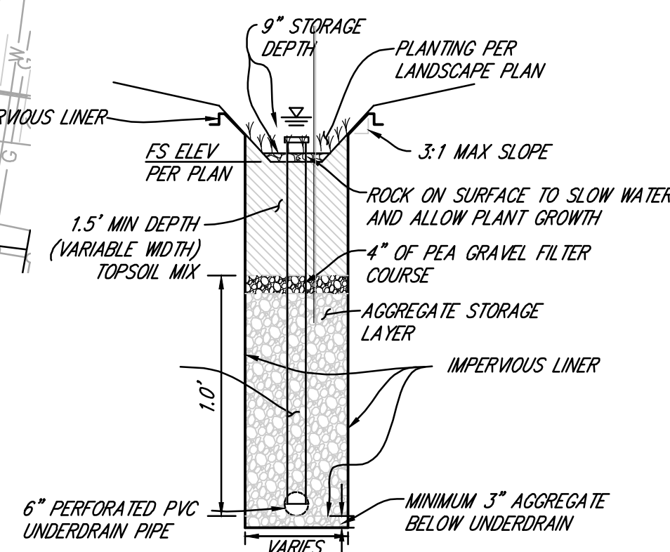
BIOFILTRATION BASIN B SECTION
